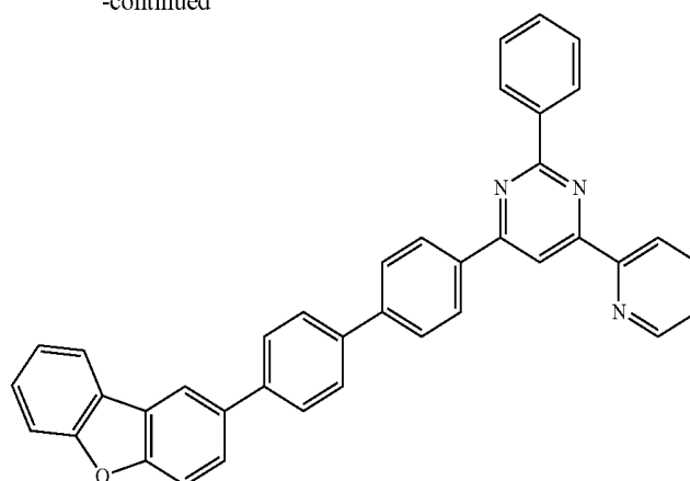
Compound 46
