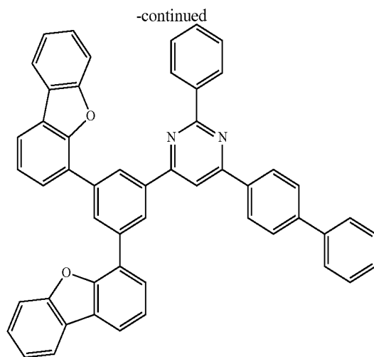
Compound 53
