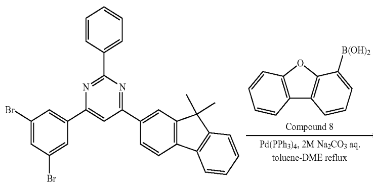
Compound 81
