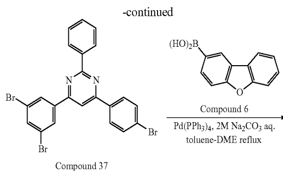
Compound 37
