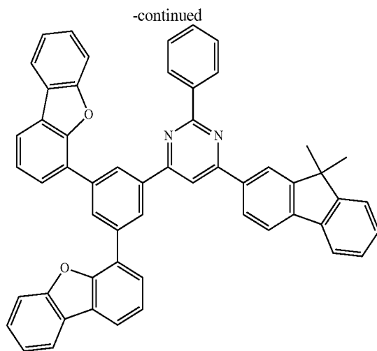
Compound 83
