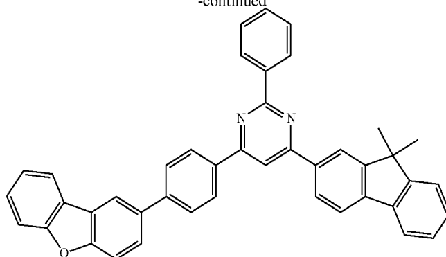
Compound 28
