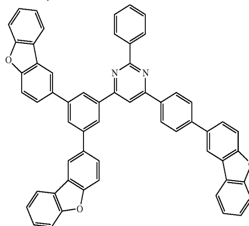
Compound 38
