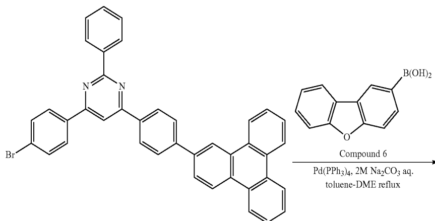
Compound 58
