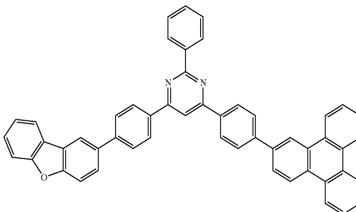
Compound 59
