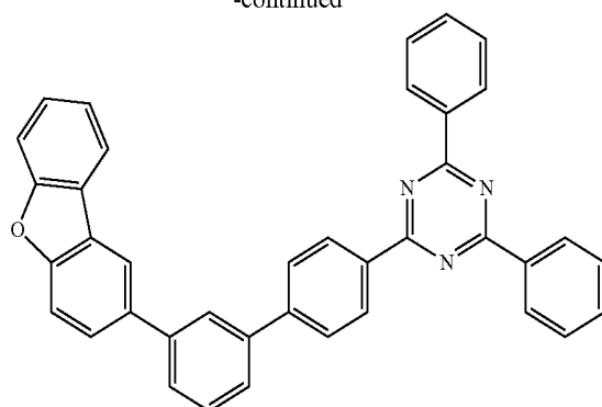
Compound 34
