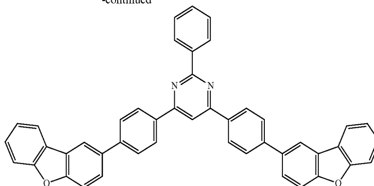
Compound 31
